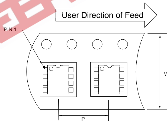
Standard Reel Component Orientation for TR Suffix Device
