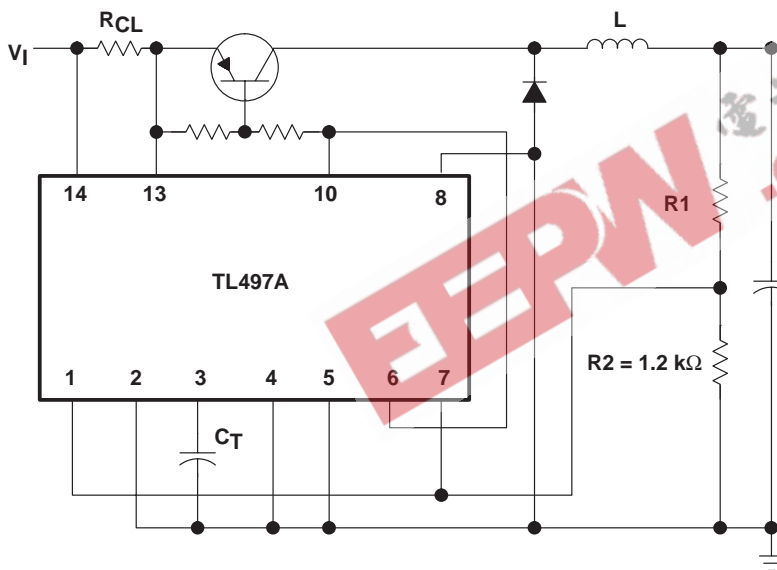
EXTENDED POWER CONFIGURATION (using external transistor)
