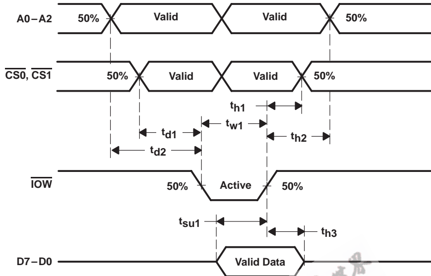
Figure 5. Write-Cycle Timing
