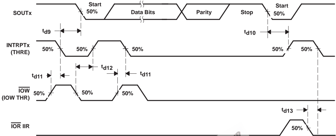
Figure 12. Transmitter Timing Waveforms
