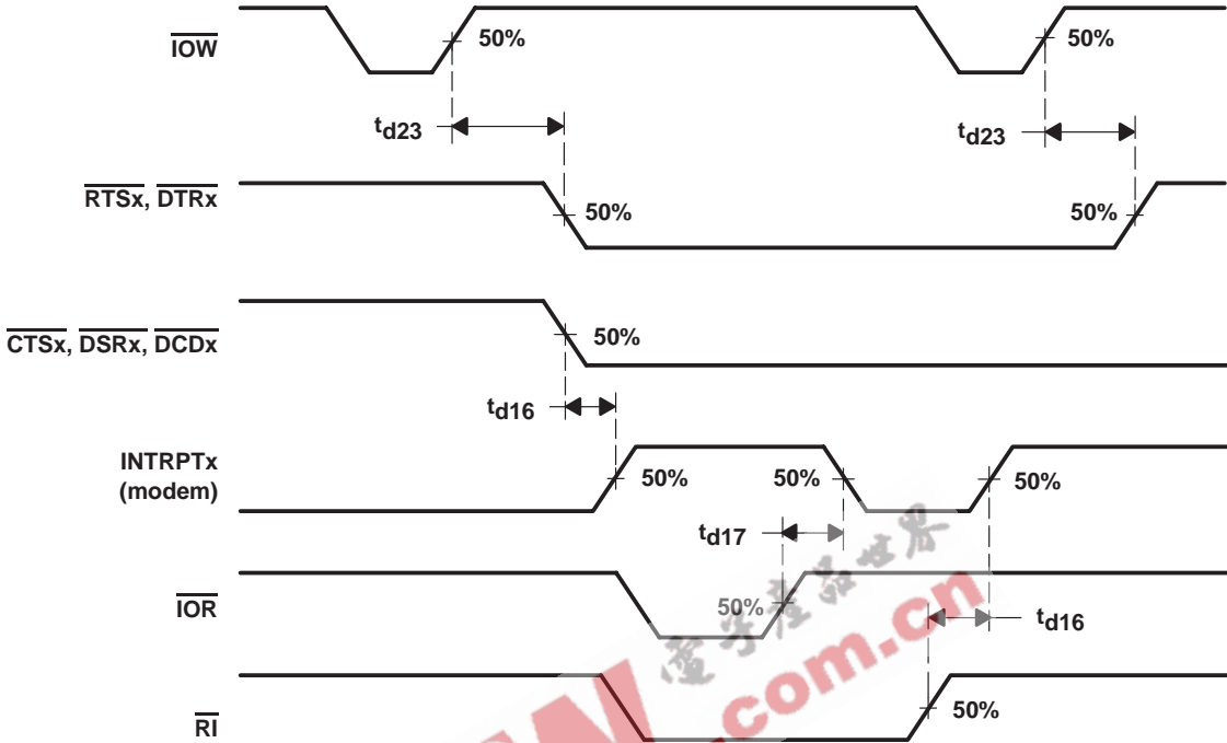
Figure 15. Modem-Control Timing
