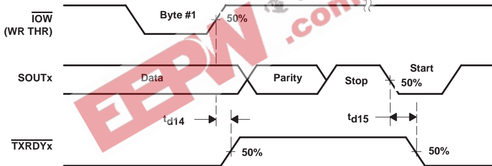
Figure 13. Transmitter Ready ( \overline{\text{TXRDYx}} ), FCR0 = 0 or FCR0 = 1 and FCR3 = 0 (Mode 0)
