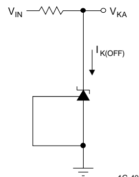
TEST CIRCUIT 3
