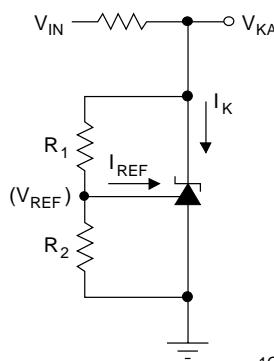
TEST CIRCUIT 2
