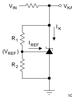
TEST CIRCUIT 2
