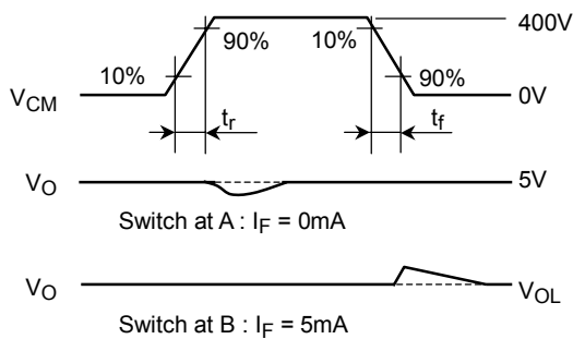
Transient Immunity and Typ. Waveforms.
