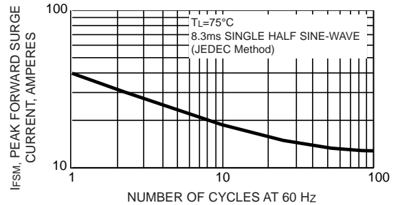
FIG. 6 - MAXIMUM NON-REPETITIVE FORWARD SURGE CURRENT
