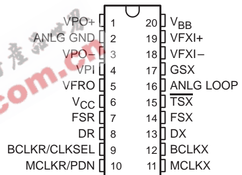
DW OR N PACKAGE (TOP VIEW)
