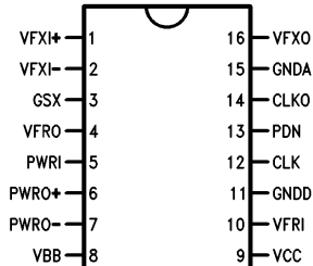
Dual-In-Line Package
