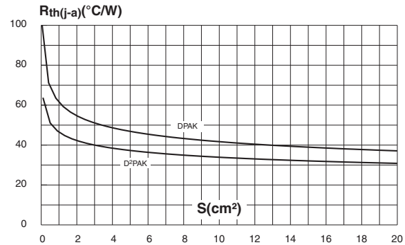
Figure 14: Thermal resistance junction to ambient versus copper surface under tab (epoxy printed circuit board FR4, copper thickness: 35µm) (DPAK and D²PAK)
