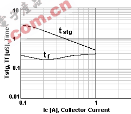
Figure 4. Switching Time
