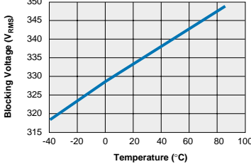
TS122 Typical Blocking Voltage vs. Temperature
