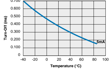
TS122 Typical Turn-Off vs. Temperature (Load Current = 170mADC)
