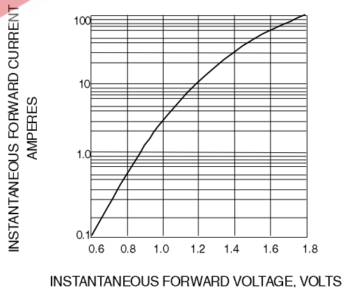
Fig. 4-TYPICAL FORWARD CHARACTERISTIC
