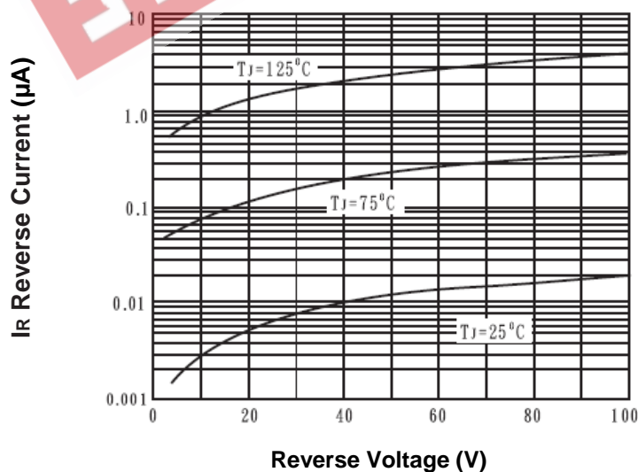
Fig.3- Typical Instantaneous Reverse Characteristics
