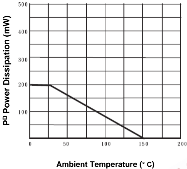
Fig.1- Forward Power Dissipation Derating Curve
