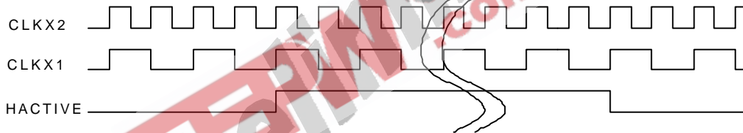
Figure 8. VIDEO HACTIVE timing
