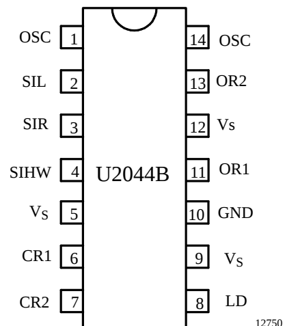
Figure 1. Pinning
