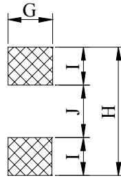
( PCB Pattern )
