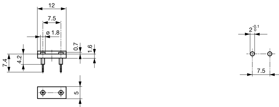
Drilling Diagram
