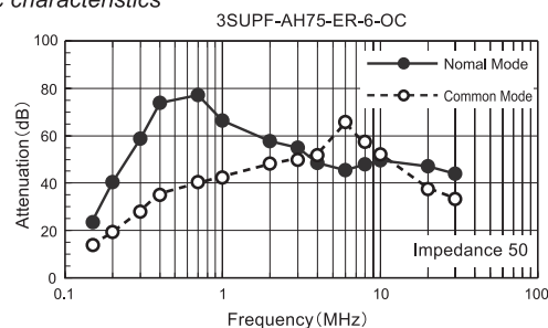
Static characteristics
