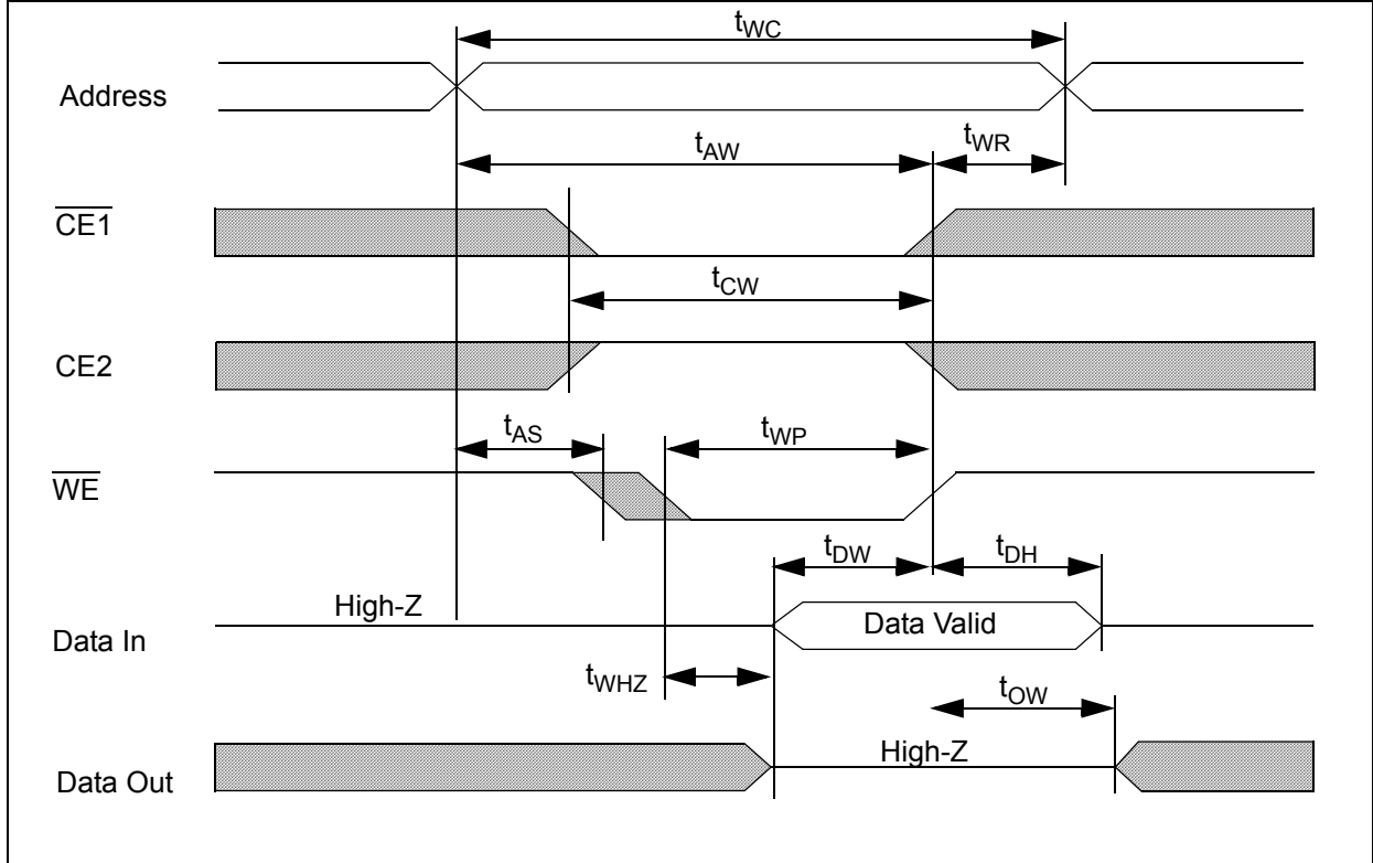
Timing Waveform of Write Cycle ( \overline{\text{CE1}} Control)
