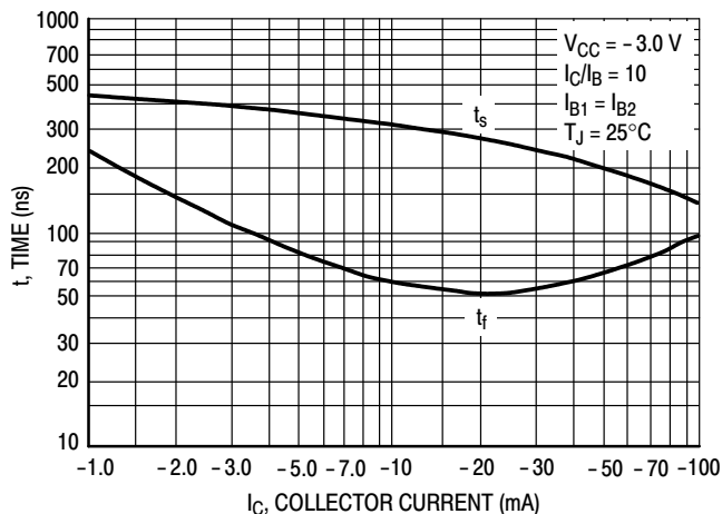
Figure 11. Turn-Off Time
