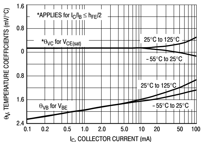
Figure 9. Temperature Coefficients
