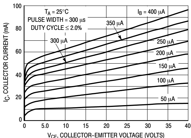
Figure 7. Collector Characteristics
