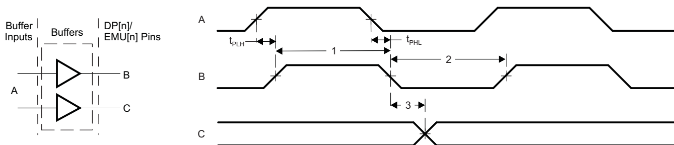
Figure 8-36. STM Trace Timing
