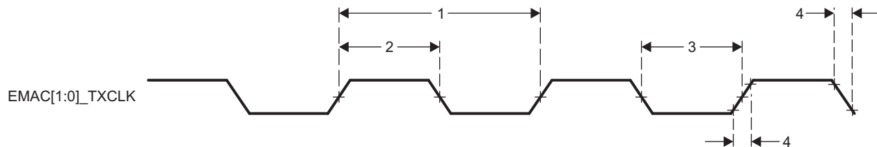
Figure 8-5. EMAC[1:0]_TXCLK Timing
