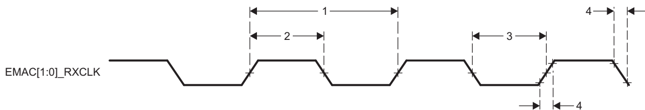
Figure 8-4. EMAC[1:0]_RXCLK Timing
