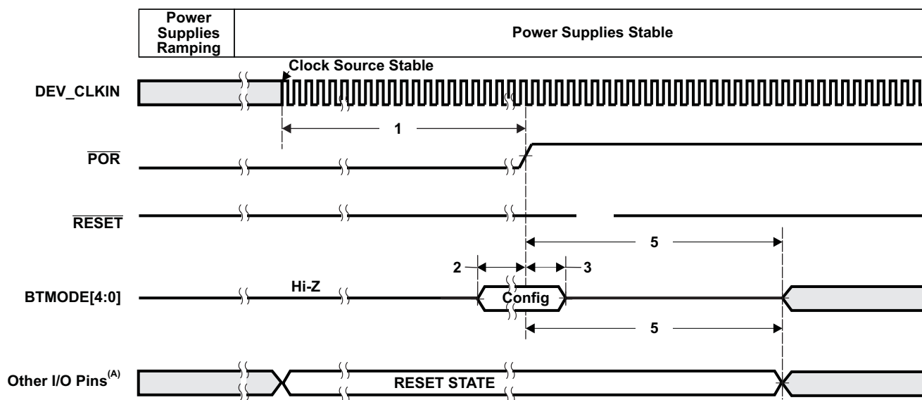
Figure 7-2. Power-Up Timing
