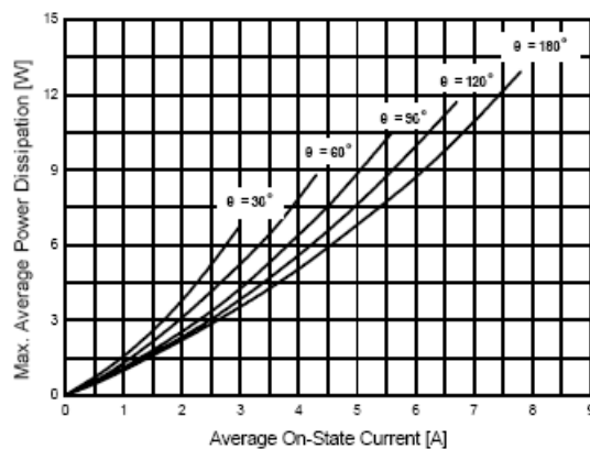
Fig.8 Power Dissipation
