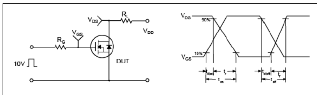
Fig.11 Resistive Switching Test Circuit & Waveform
