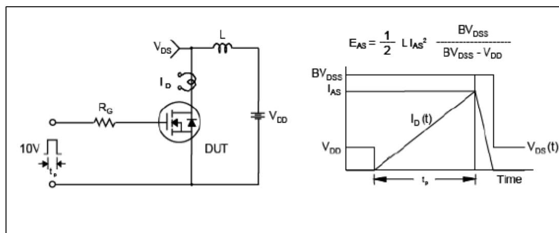
Fig.12 Uncamped Inductive Switching Test Circuit & Waveform
