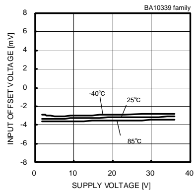
Fig. 28 Input Offset Voltage - Supply Voltage
