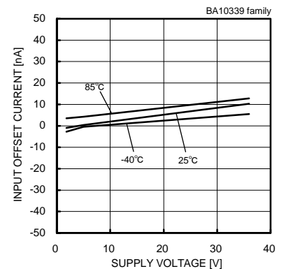
Fig. 32 Input Offset Current – Supply Voltage
