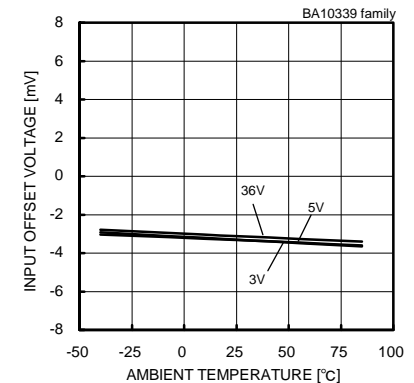
Fig. 29 Input Offset Voltage – Ambient Temperature
