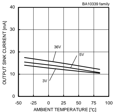
Fig. 27 Output Sink Current - Ambient Temperature (VOU=1.5[V])
