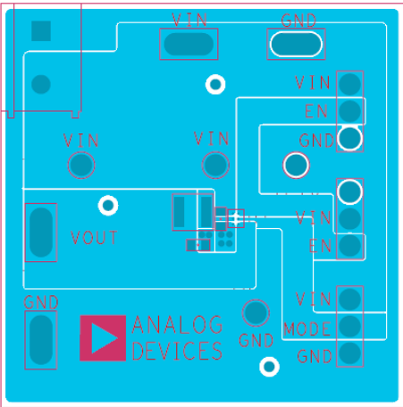
Figure 36. Top Layer
