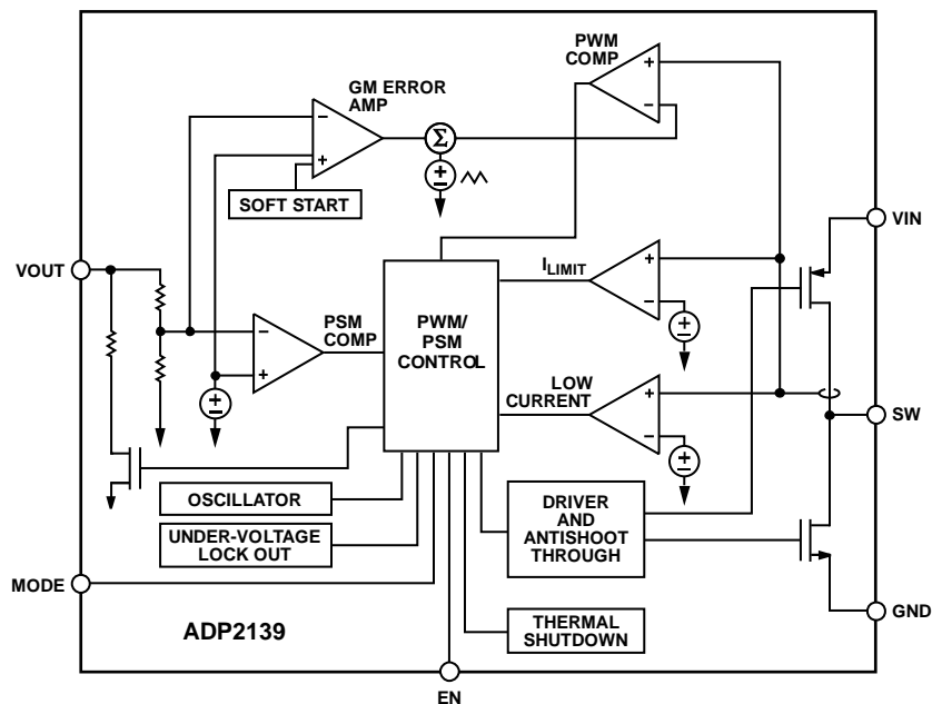
Figure 33. ADP2139 Functional Block Diagram
