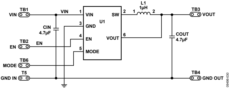
Figure 35. Evaluation Board Schematic
