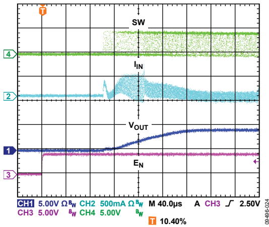
Figure 28. Startup, V_{OUT} = 0.8V , I_{OUT} = 10mA
