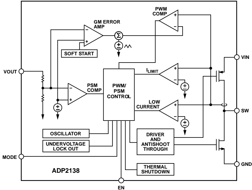
Figure 32. ADP2138 Functional Block Diagram
