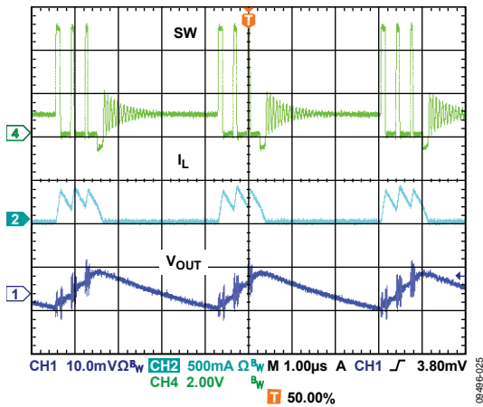
Figure 29. Typical Waveform, V_{OUT} = 1.8V , PSM Mode, I_{OUT} = 10mA
