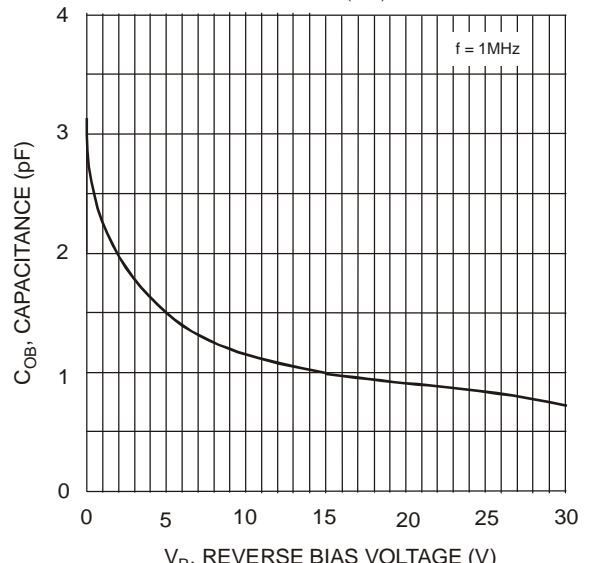
Fig. 4 Output Capacitance
