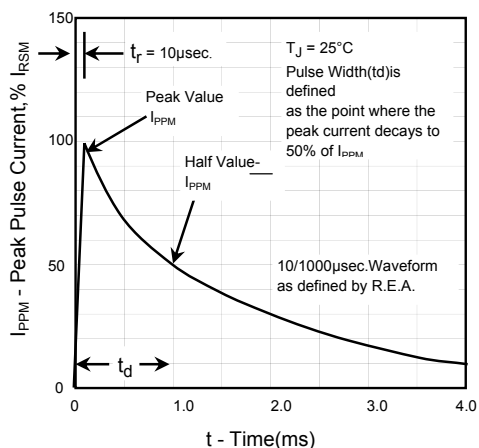
Fig.3 Pulse Waveform
