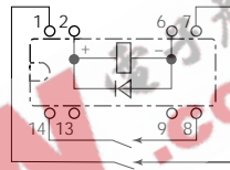
DPST-2 Form A w/diode
