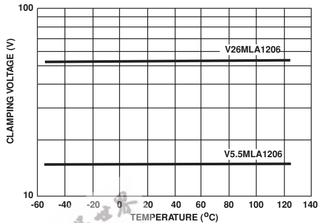
FIGURE 12. CLAMPING VOLTAGE OVER TEMPERATURE (V C AT 10A)
