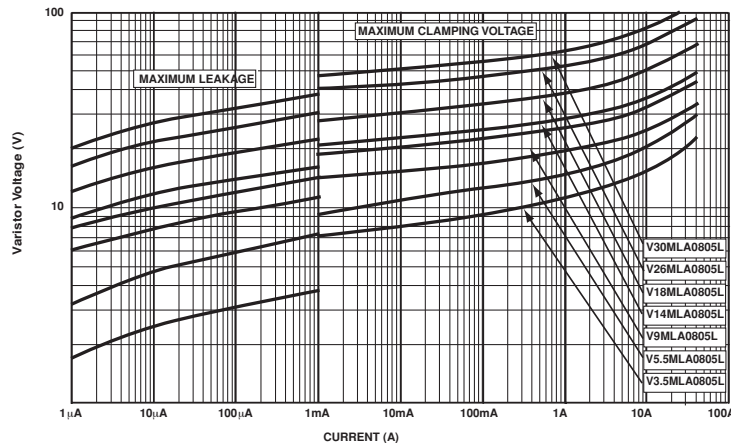
FIGURE 6. LIMIT V-I CHARACTERISTIC FOR V3.5MLA0805L TO V30MLA0805L
