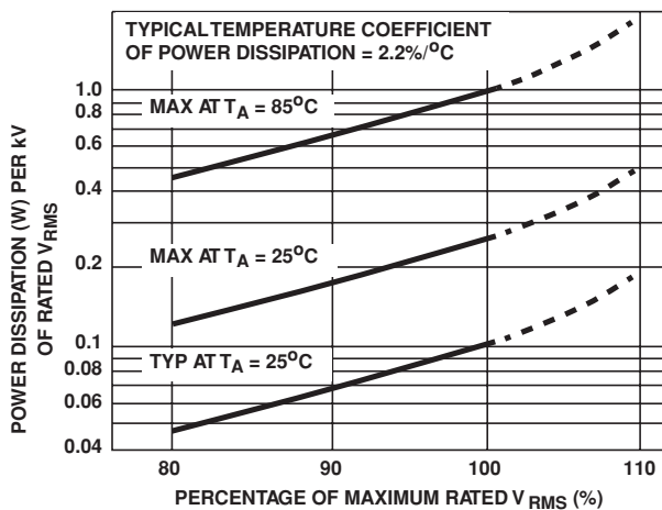
FIGURE 3. STANDBY POWER DISSIPATION vs APPLIED V_{RMS} AT VARIOUS TEMPERATURES
