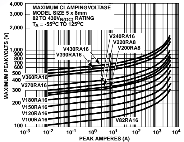
FIGURE 6. CLAMPING VOLTAGE FOR V82RA16 - V430RA16
