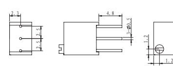
WIW1015-Y
