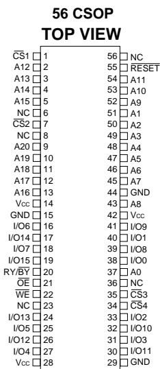
FIG. 1 PIN CONFIGURATION FOR WF4M16-XDTX5
