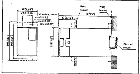
EXTERNAL DIMENSION
