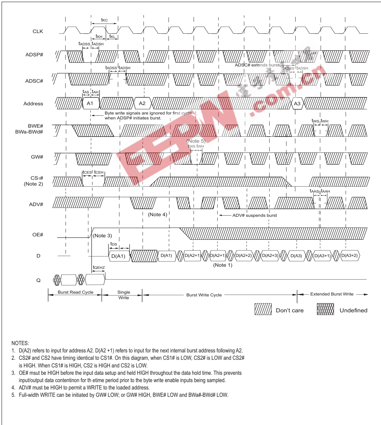
FIGURE 3 – WRITE TIMING
