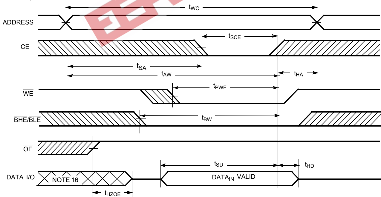
Write Cycle No. 2 (CE Controlled) [10, 14, 15]
