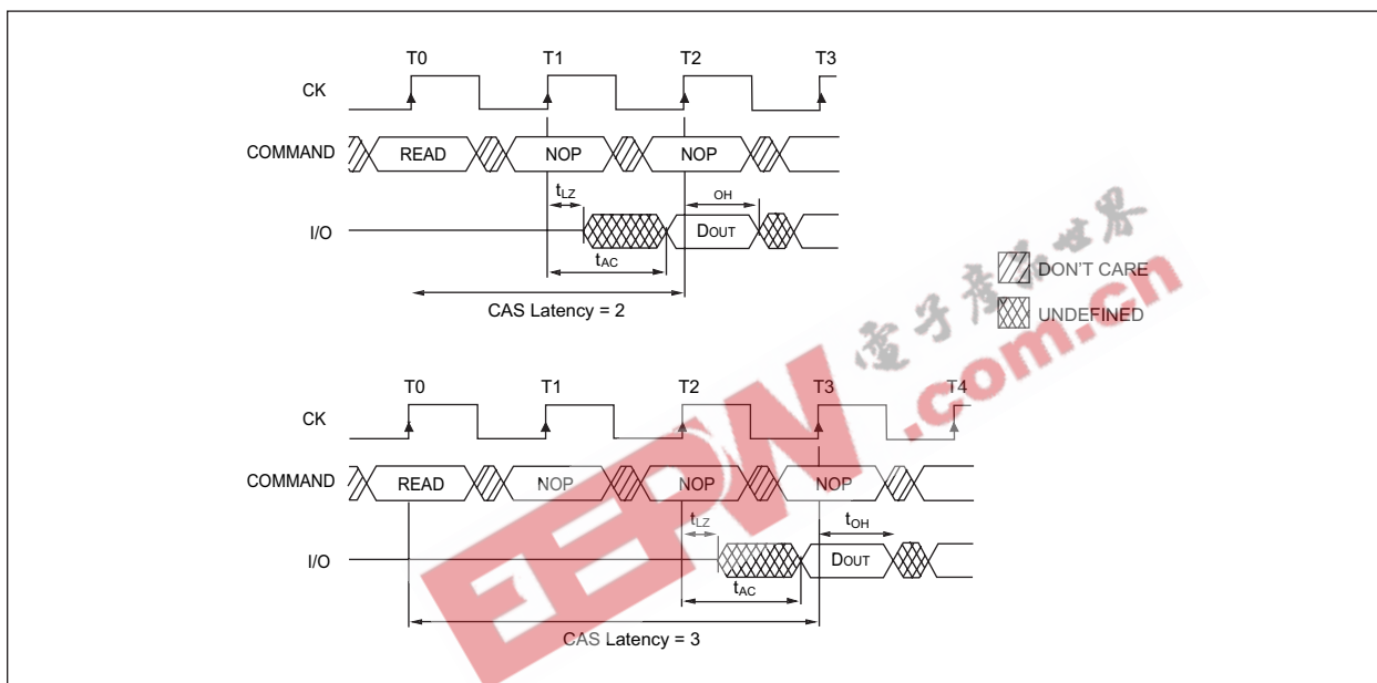
FIGURE 4 – CAS LATENCY
