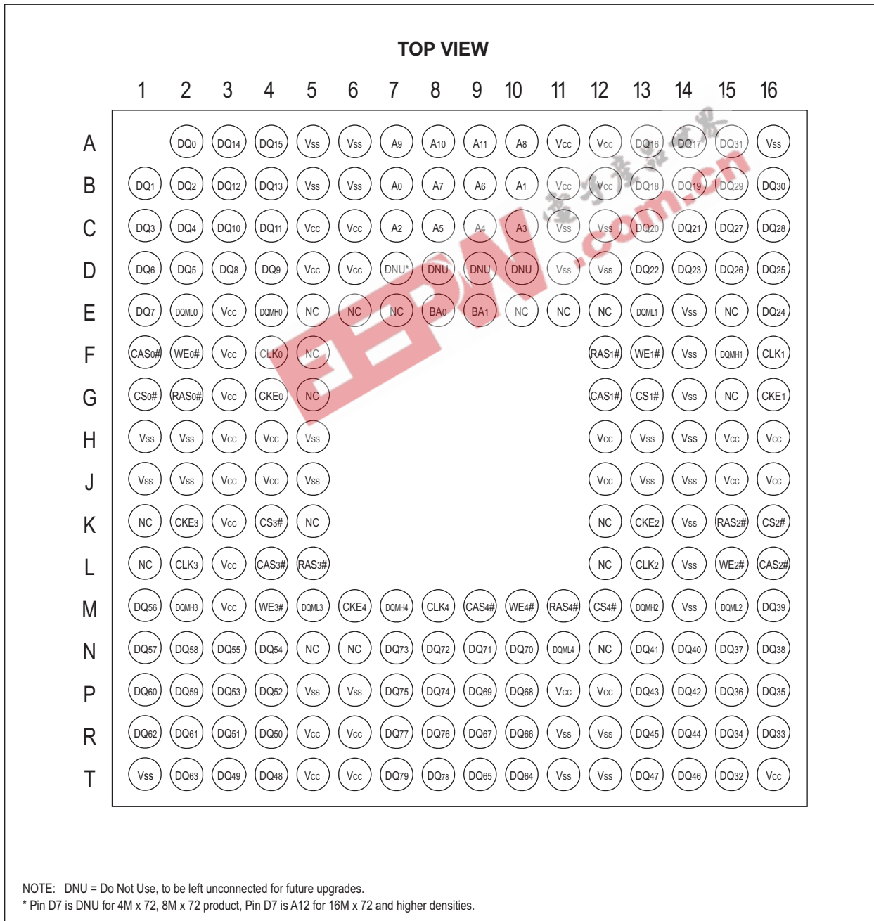
FIGURE 1 – PIN CONFIGURATION
