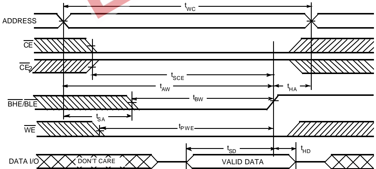
Write Cycle 4 (BHE/BLER Controlled, OE LOW) [17, 18]
