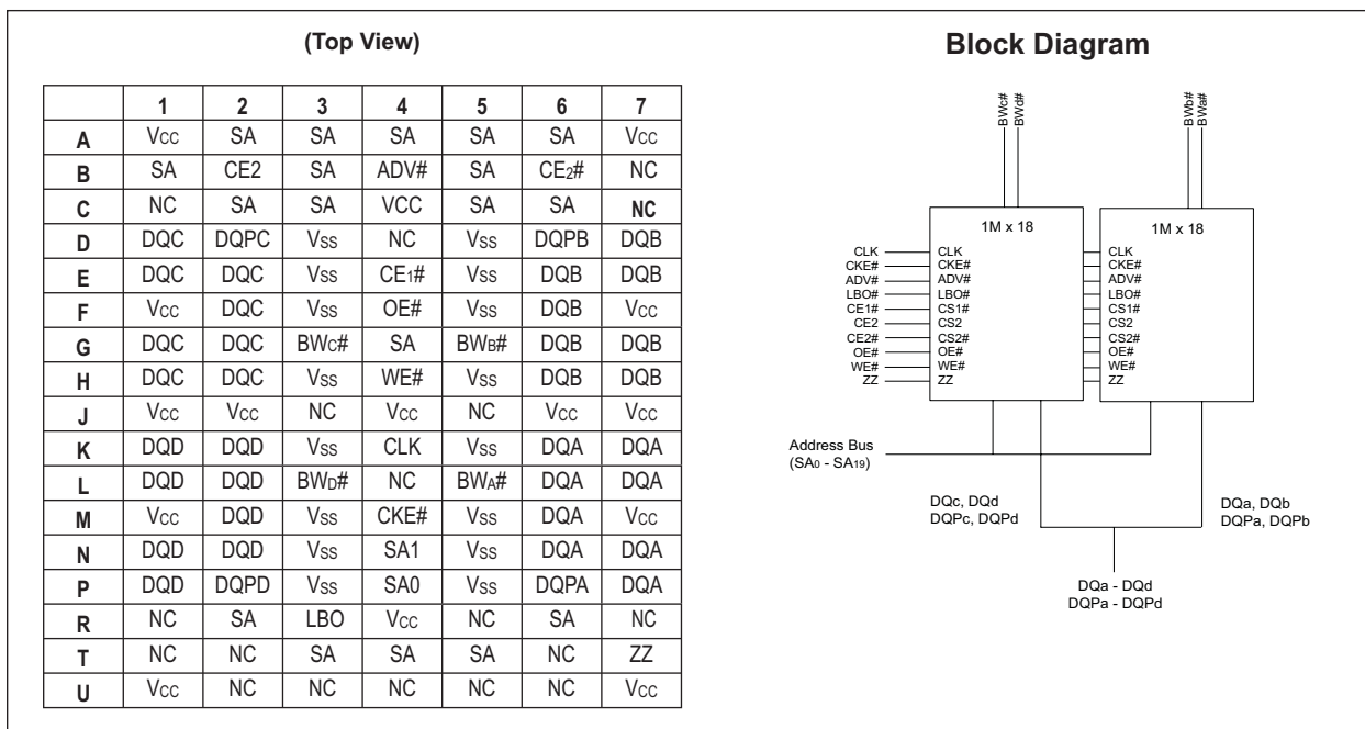
FIGURE 1 – PIN CONFIGURATION
