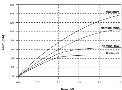
FIGURE A – PULL-DOWN CHARACTERISTICS
