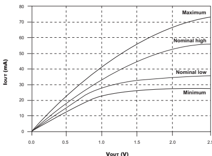
FIGURE C – PULL-DOWN CHARACTERISTICS
