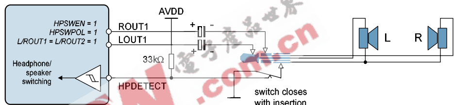
Figure 10 Example Headset Detection Circuit Using Normally-Closed Switch
