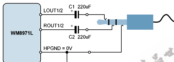
Figure 11 Recommended Headphone Output Configuration
