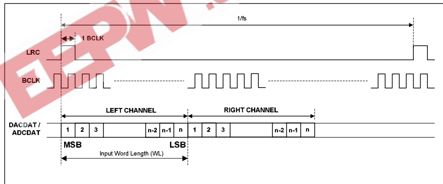
Figure 21 DSP/PCM Mode Audio Interface (mode B, LRP=1, Master)
