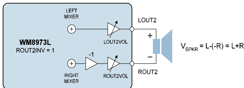
Figure 12 Speaker Output Connection
