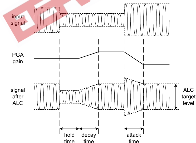
Figure 8 ALC Operation
