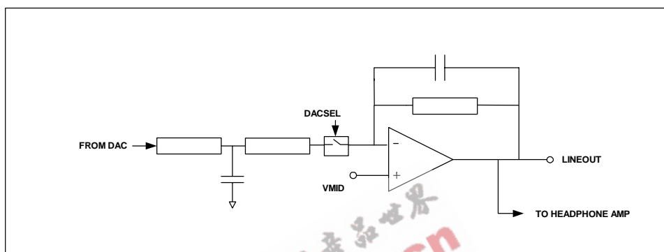
Figure 14 Line Output Schematic
