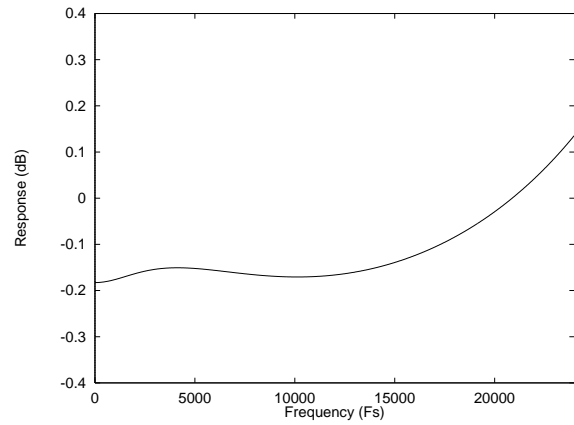
Figure 37 De-Emphasis Error (48kHz)
