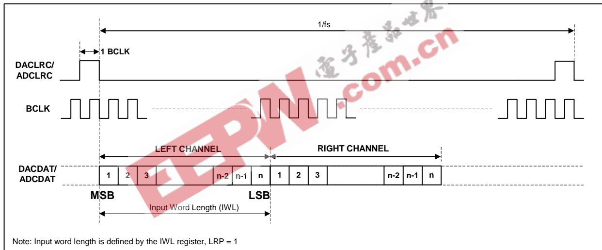
Figure 19 DSP Mode
