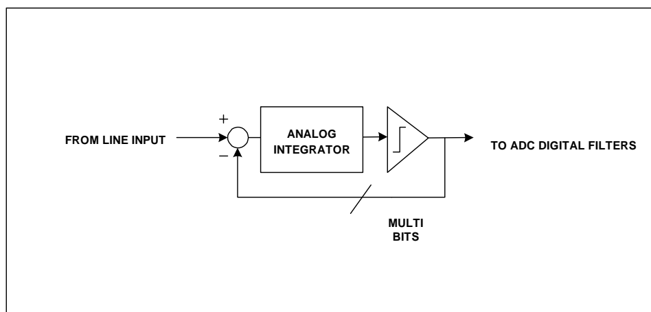
Figure 10 Multi-Bit Oversampling Sigma Delta ADC Schematic
