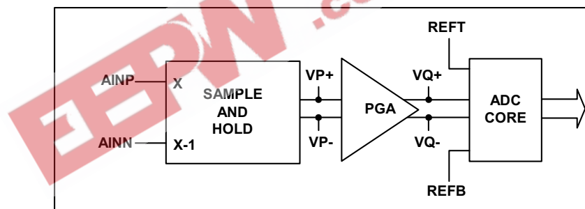
Figure 2 Analogue Input Signal Flow
