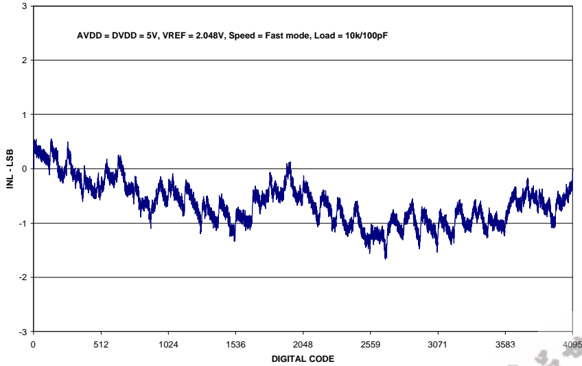
Figure 2 Integral Non-Linearity
